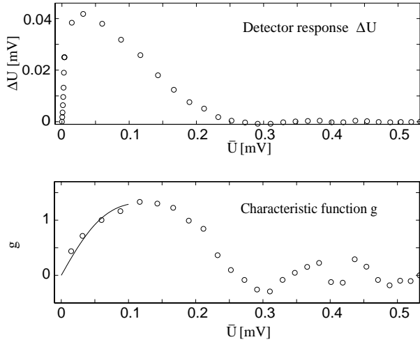
Figure 3: Upper graph: The detector response \Delta U as a function of \bar{U} . Lower graph: The characteristic function g , as defined by Equation (3), plotted versus \bar{U} . The solid line shows an extrapolation of g for small \bar{U} .
