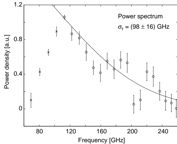
Figure 4: The coherent radiation spectrum as obtained from a discrete Hilbert transform of the characteristic function g .
