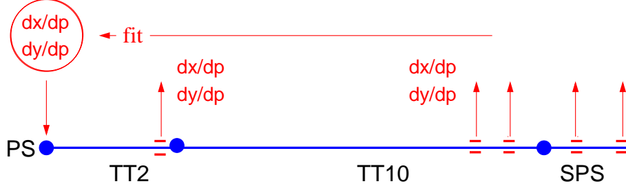
Figure 2: Schematic representation of the dispersion measurement.
