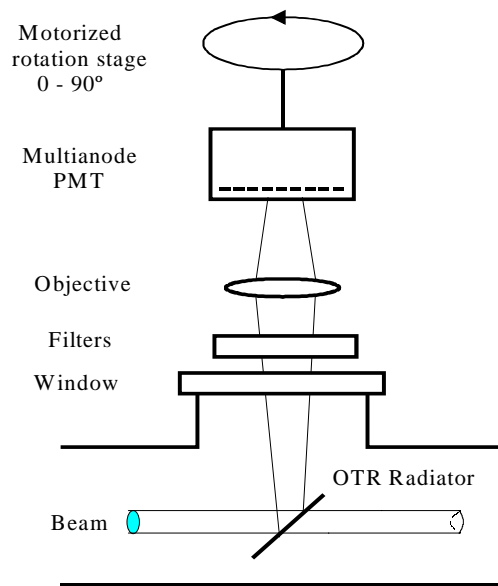
Figure 1: Schematic set-up of the bunch-by-bunch OTR monitor in TT10.
