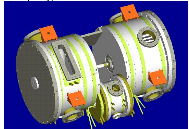
Fig 6: Assembled CCDTL prototype.
