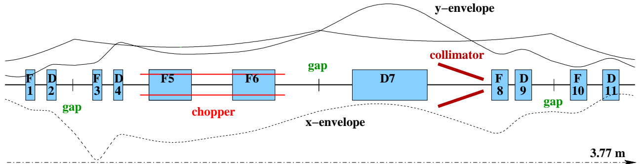
Fig. 1: Chopper line and beam envelopes from TRACE3D
