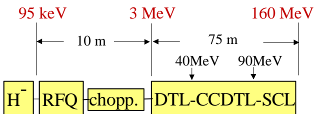
Fig. 2: The Linac4 schematic layout
