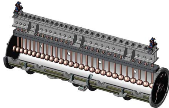
Figure 2: Cut of DTL tank 1 prototype.
