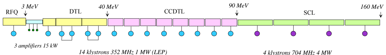
Figure 3: Linac4 RF-power distribution.
