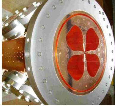
Figure 1: The 2 nd RFQ module after final brazing.
