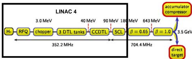
Figure 1: SPL Layout.
