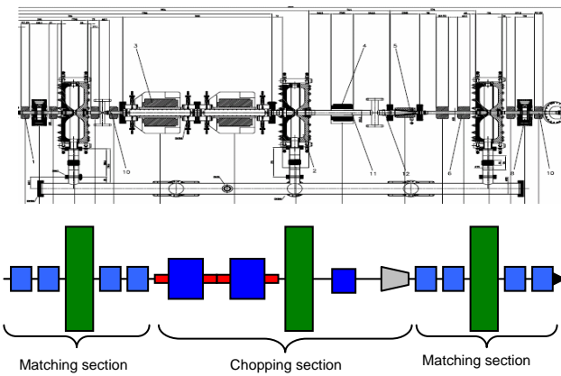
Figure 2 : Chopper-line layout
