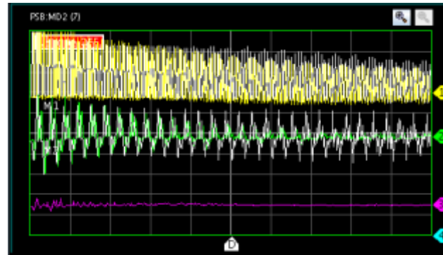
Figure 5: 0.7 turns injected with an oscillation of \sim 25 mm peak-to-peak. Top: sum signal; below: difference signal. The stored larger amplitude signal is for a beam without sieve; the superimposed smaller amplitude signals are measurements for a beam with sieve ( \sim 5 times less dense; vertical scale of scope was changed). Note the significant difference in signal damping.
