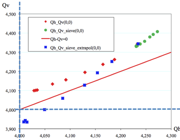
Figure 3: Tunes for particles having only small amplitude oscillations at the start of acceleration. Lozenges: without sieve; circles: with sieve; squares: extrapolated tunes using the number of particles without sieve and the emittances obtained with sieve. The solid line represents the linear coupling resonance Q_h-Q_v=0 , the dotted lines the integer resonances.
