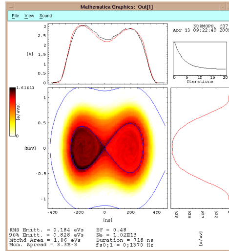
Figure 1: Tomographic reconstruction of the longitudinal phase space of an ISOLDE beam 100 ms after injection; a bunching factor BF close to 0.5 is achieved combining h=1 and h=2 systems.
