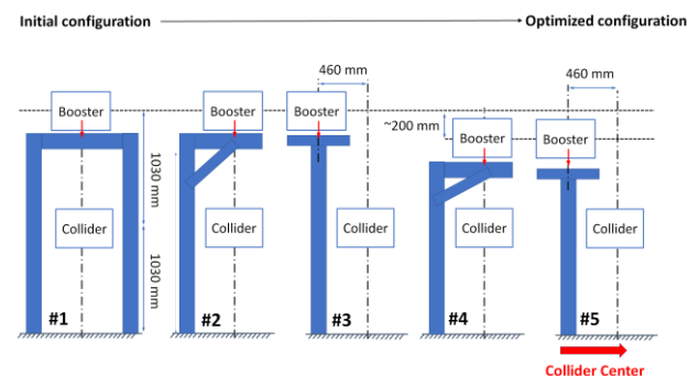
Fig. 3. Principles of optimization of the booster placement and supporting system.
