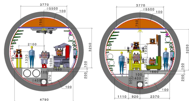
Fig. 1. Configurations for the relative placement between booster and collider. Left: horizontal configuration. Right: vertical configuration.
