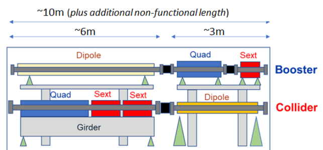
Fig. 6. Preliminary proposal for an arc-half cell mock-up layout.
