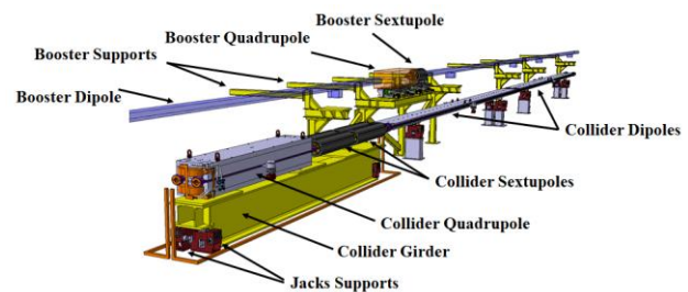
Fig. 4. CAD model of arc cell, with focus on the Short Straight Section.
