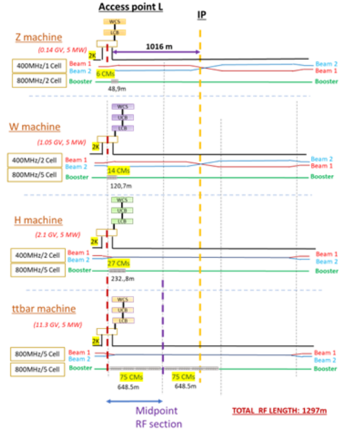
Figure 6: RF and Cryogenic Layout point L - 2023
